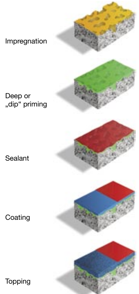
Graphic illustration of an impregnation, deep or „dip“ priming, a sealant, a coating and a topping with Silikal
